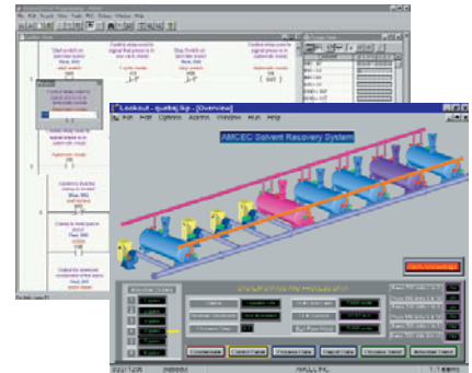
Directsoft RLL programming and PC-based HMI (such as LookoutDirect) over Ethernet to multiple PLCs
